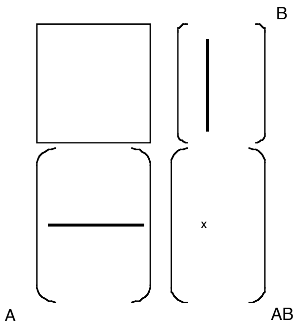
Figure 39. Multiplier les matrices
